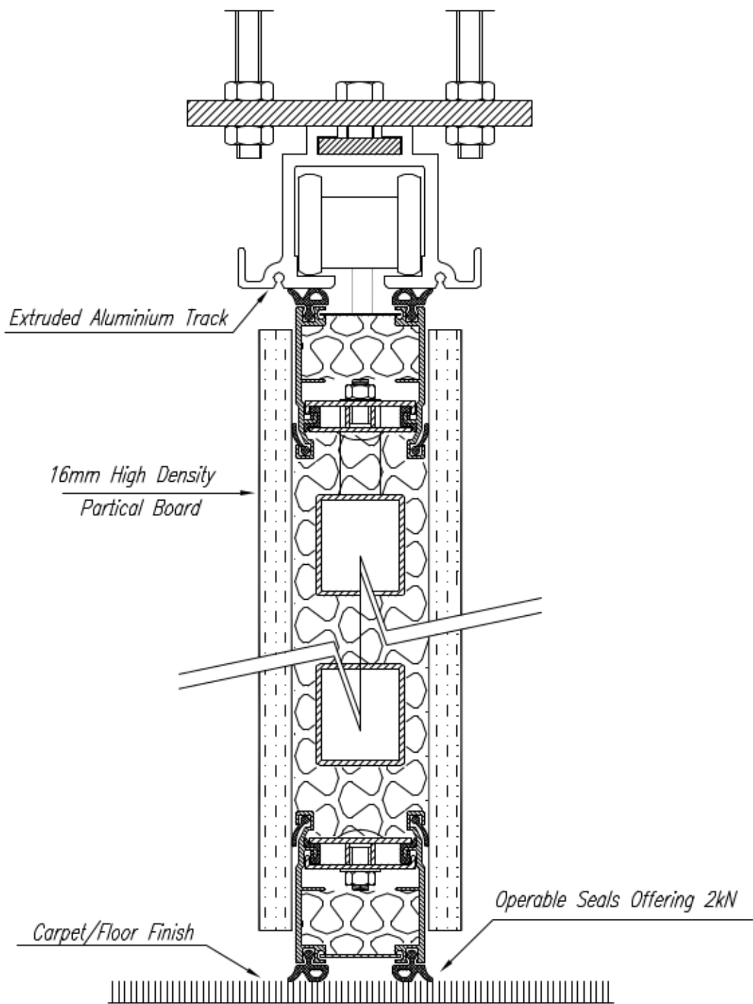
Single Point Track with Trolley
