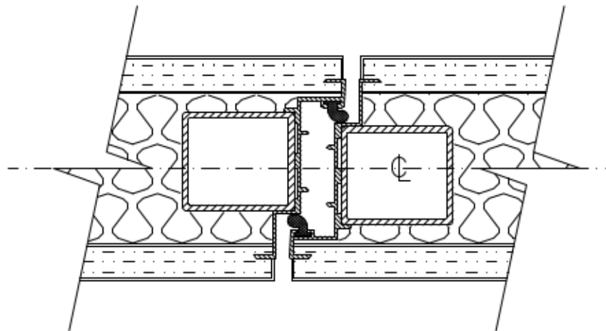
CLOSURE DETAIL
